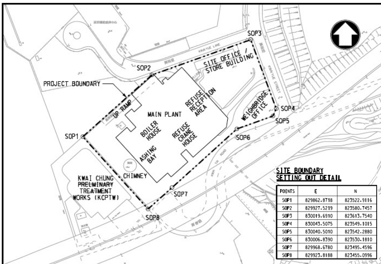
INSET : LAYOUT OF KWAI CHUNG INCINERATION PLANT
